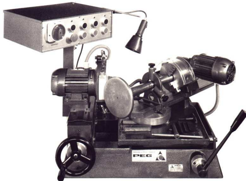
Valve refacer for big motors. Up to Ø40mm valve stem capacity.
