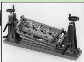
Two towers secure to the mill bed and support the cradle assembly
